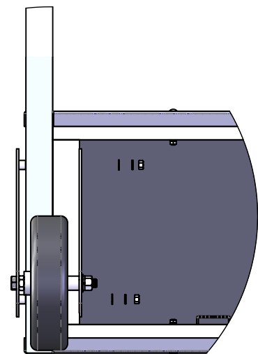
BACK VIEW WHEEL KIT ASSEMBLY
