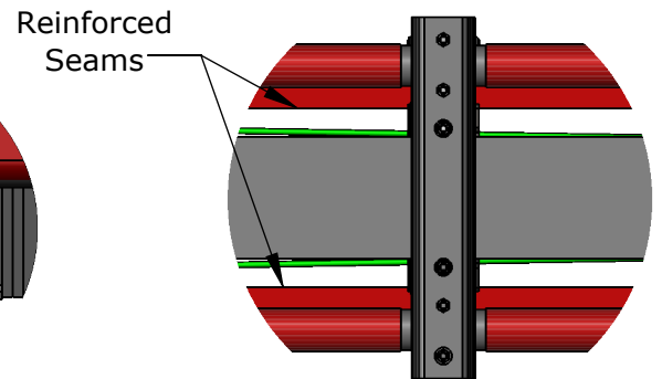
DETAIL C Solid Vinyl Mounting, Typical on Both Sides of Structure
